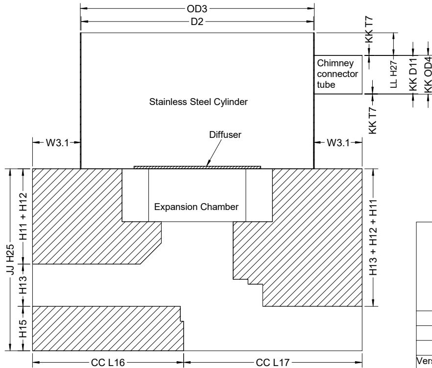
Section L-L
