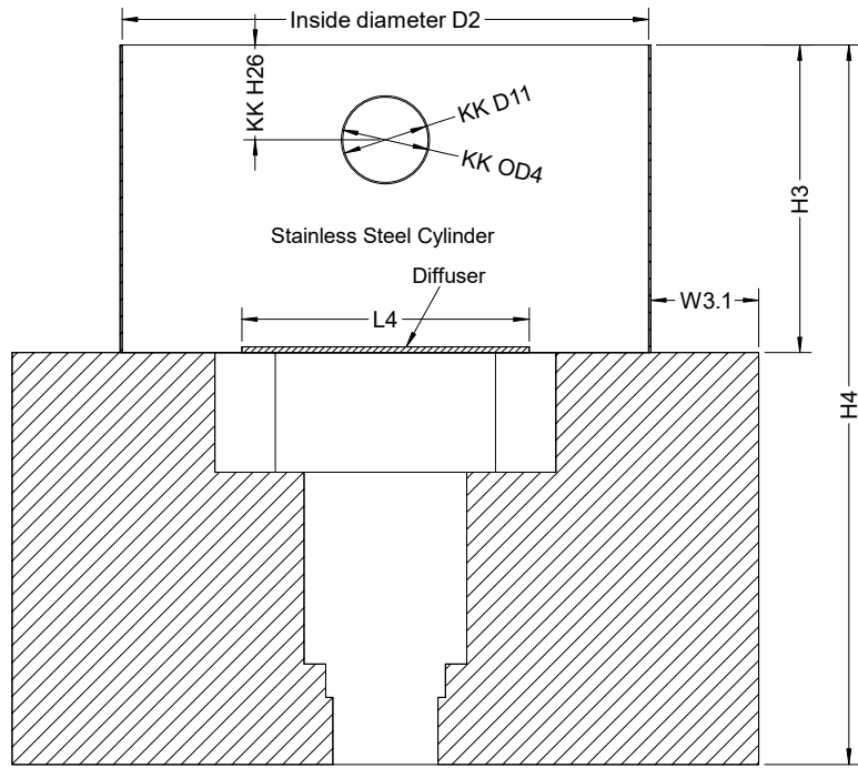
Section K-K
