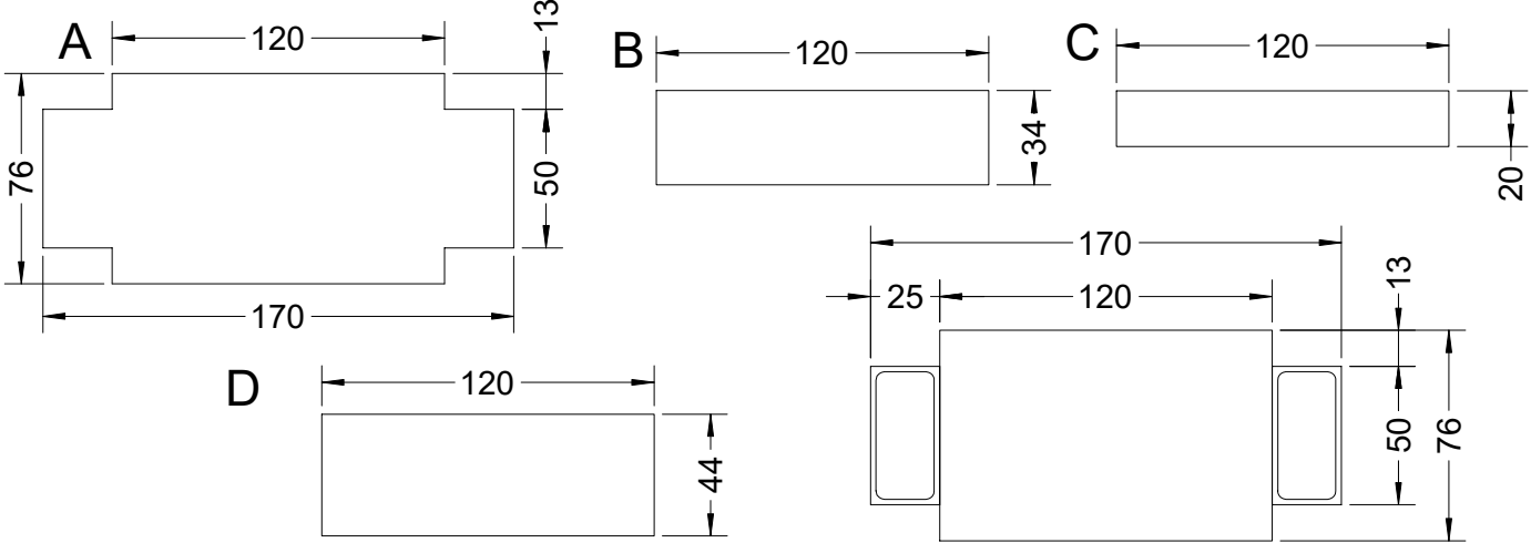
Bridge - 3mm welded
