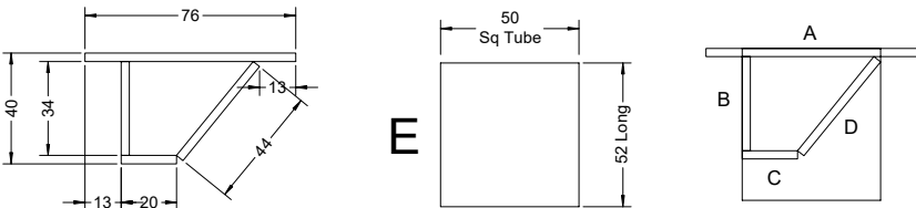
Bridge - 3mm welded
