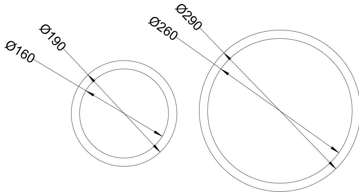
Cooking hole supports rings Material 2mm mild steel
