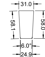
Inside Form
