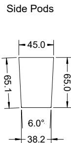
Outside Form
