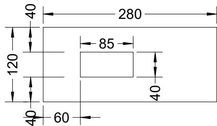
Door Panel For Left-open turn upside down
