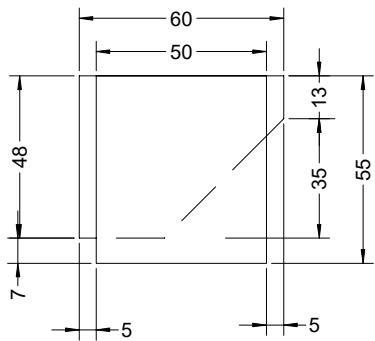
End view
