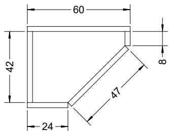
Bridge - 3mm welded
