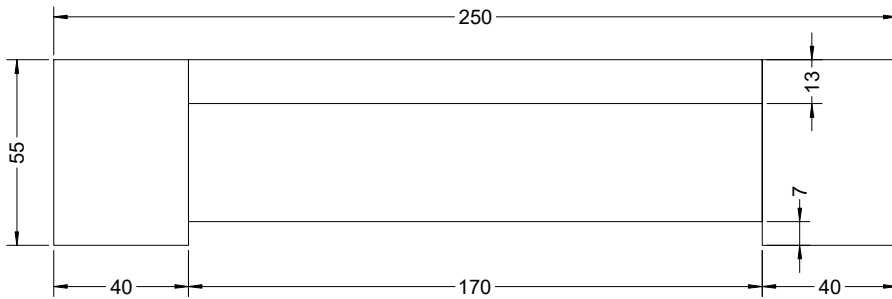
Bridge - Cast Iron
