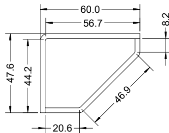
Bridge - 3mm bent
