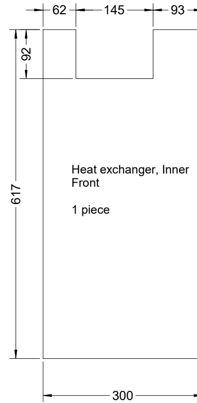
Inner shell Front plate
