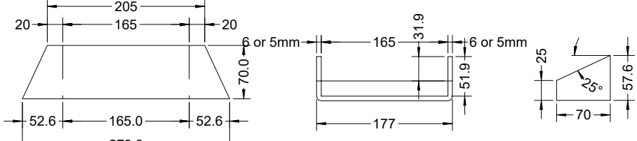
1 Grate Support Bracket
