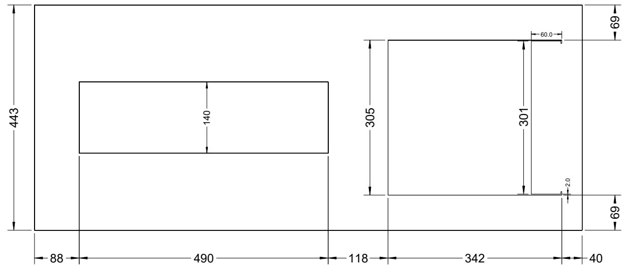
Bottom Plate, Fits inside front, back and sides
